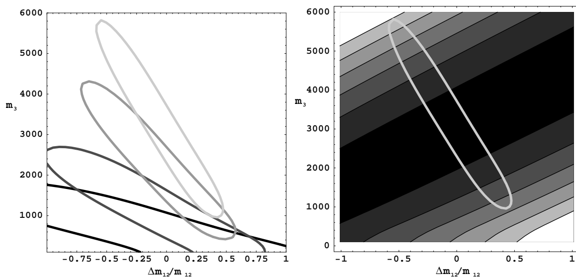
Figure 7: Case V f = 1000 GeV: In these plots, the angle s_{23}^d = 1/\sqrt{2} , while the other angles are set to zero. In the plot on the left, the contours, from darkest to lightest, are for m_{12} = 500, 1000, 2000, 3000 GeV, and show the constraints from the K , B_d , and D systems. In the plot on the right, we overlap the constraint contour for m_{12} = 3000 GeV with a plot of the enhancement in the B_s mass splitting relative to the SM contribution. From darkest to lightest, this enhancement is a factor of 2, 4, 6, 8, 10, and 12, respectively.
