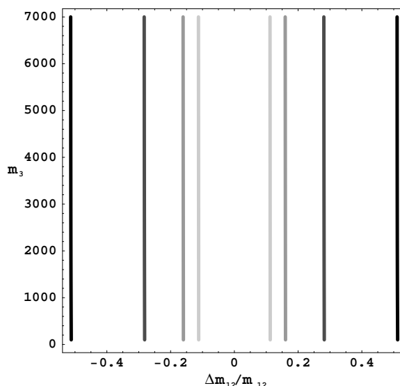
Figure 4: Case II f = 1000 GeV: In this plot, we show the results for the case where V_{Hd} = \mathbf{1} . Again, from darkest to lightest, the average mass of the first two generations increases as m_{12} = 500, 1000, 2000, 3000 GeV. In this scenario, only the D system is affected, and so the contours correspond to the points at which the T-odd fermion contributions exceed the experimental upper bounds.
