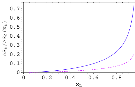
Figure 2: \Delta S_t/S_0(x_t) versus x_L for different values of f , f = 1 TeV (solid) and f = 2 TeV (dashed). \mathcal{O}(v^4/f^4) corrections are included to show the large x_L behavior.
