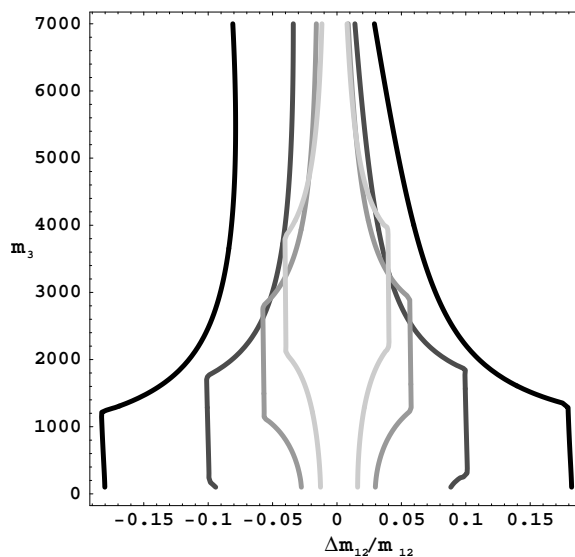
Figure 3: Case I f = 1000 GeV: In these plots, V_{Hd} = V_{CKM} . In order of the darkest contours to lightest, the average mass of the first two generations varies through m_{12} = 500, 1000, 2000, 3000 GeV. The D system imposes no constraints in this scenario.
