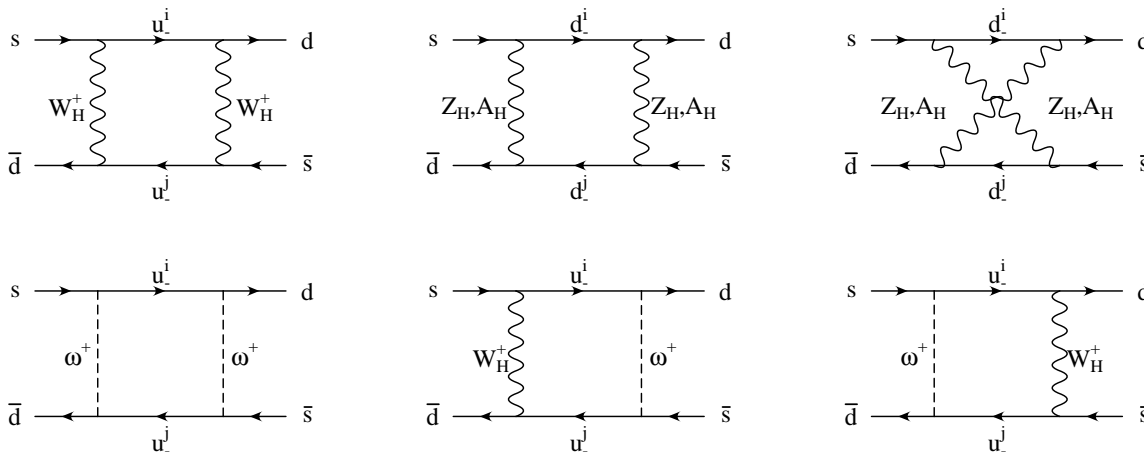
Figure 1: Box diagrams involving T-odd gauge bosons and scalars that contribute to particle anti-particle mixing in the littlest Higgs model with T-parity. There are other diagrams, such as those with two neutral scalars running in the loop. These, however, sum to zero. We show only the classes of diagrams which contribute to the functions given in the appendix.
